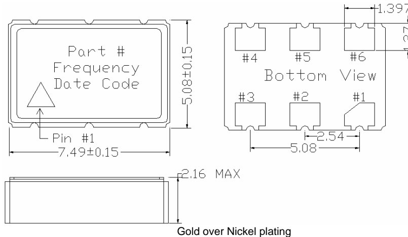
Figure 3 Optional VCC6-QAx Package Drawing
