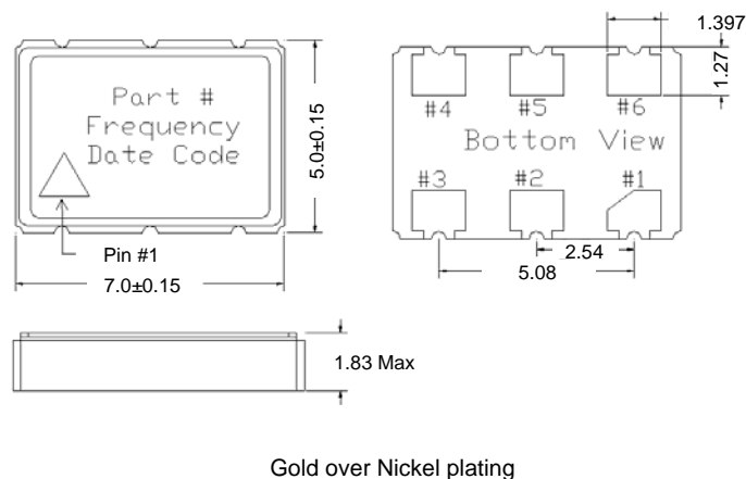
Figure 4. VCC6-QCx and VCC6-QAx Package Drawing
