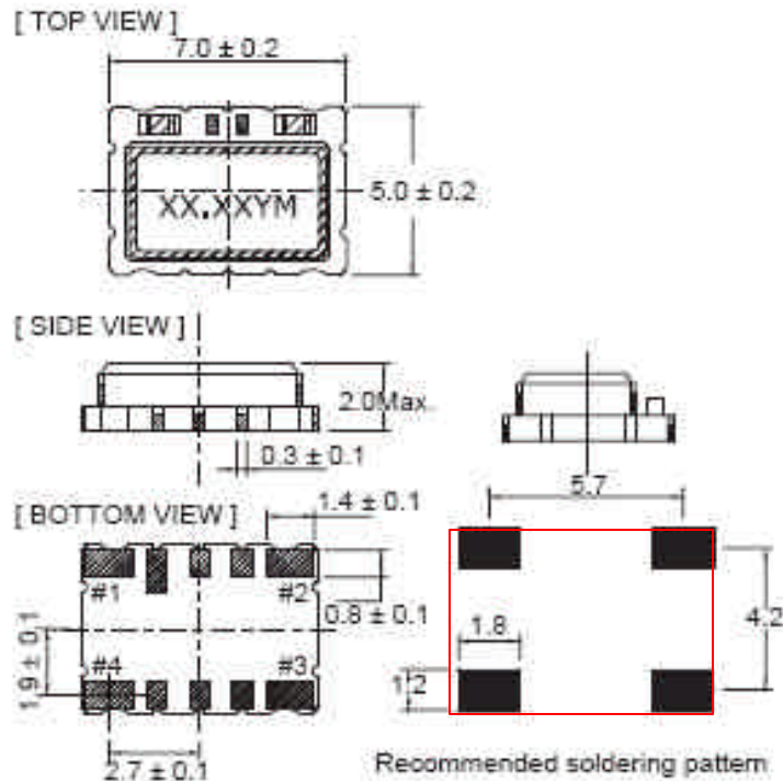
Figure 3, Package drawing
